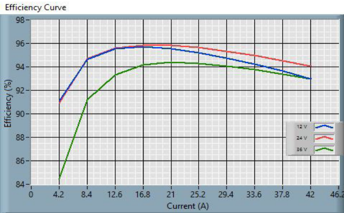
Figure 8: 24S24.42FXP (ROHS) Efficiency Curve
