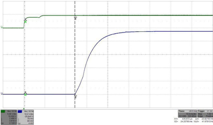
Figure 32: Turn-on by ON/OFF transient ( V_{in} applied) at full rated load current (resistive). Top trace (C1): ON/OFF signal, Bottom trace (C4): Output voltage
