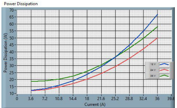
Figure 11: 24S28.36FXP (ROHS) Power Dissipation
