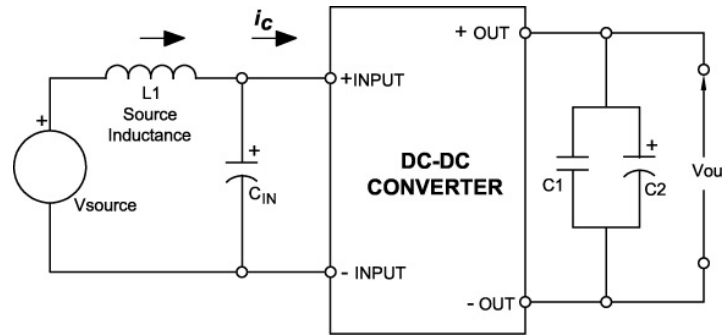
Figure 6: Test setup for measuring input reflected ripple currents i_c .
