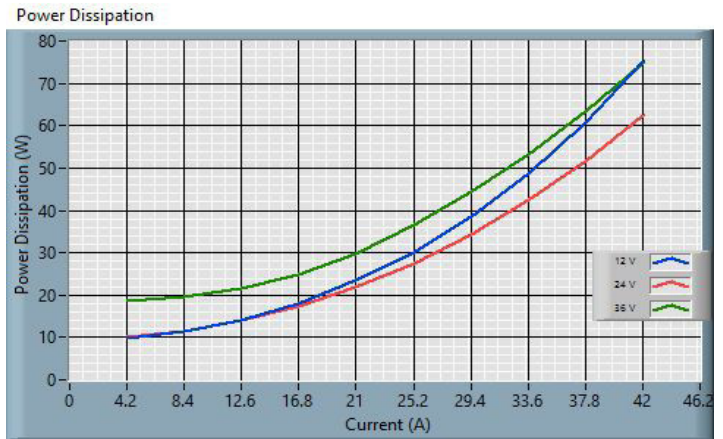
Figure 9: 24S24.42FXP (ROHS) Power Dissipation
