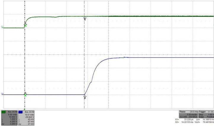
Figure 26: Turn-on by ON/OFF transient ( V_{in} applied) at full rated load current (resistive). Top Trace (C1): ON/OFF signal, Bottom Trace (C4): Output voltage.
