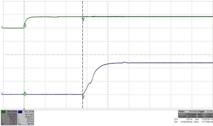
Figure 20: Turn-on by ON/OFF transient (with V_{in} applied) at full rated load current (resistive load). Top trace (C1): ON/OFF signal, Bottom trace (C4): Output voltage
