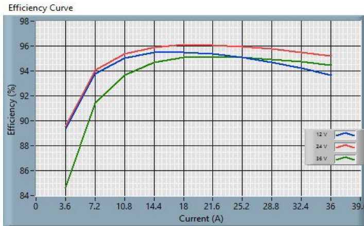
Figure 10: 24S28.36FXP (ROHS) Efficiency Curve
