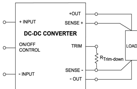
Figure 4: Circuit Configuration for Trim-Down Function
