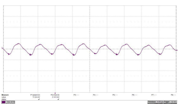
Figure 25: Input reflected ripple current, i_c (500mA/mV), measured at input terminals at full rated load current. RMS input ripple current i_c = 3.14 \times 0.5A = 1.07 A_{RMS} . (See Figure 5)
