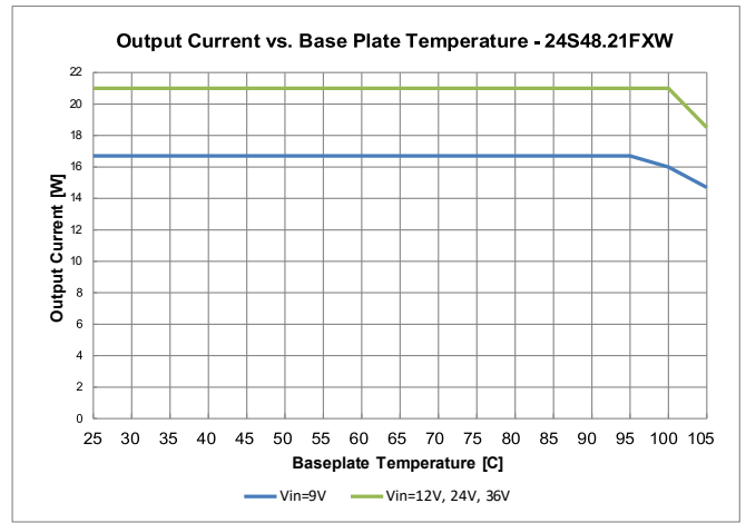
Figure 25: 24S48.21FXW (ROHS) Derating Curve
