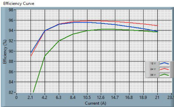
Figure 14: 24S48.21FXW (ROHS) Efficiency Curve
