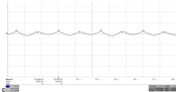
Figure 50: Output voltage ripple (100 mV/div.) at full rated load current into a resistive load at V_{in} = 24V . Time: 2 \mu s / div.
