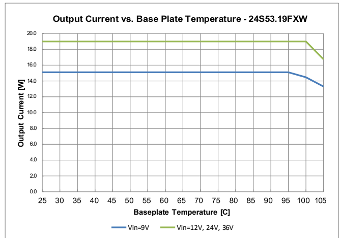
Figure 27: 24S53.19FXW (ROHS) Derating Curve
