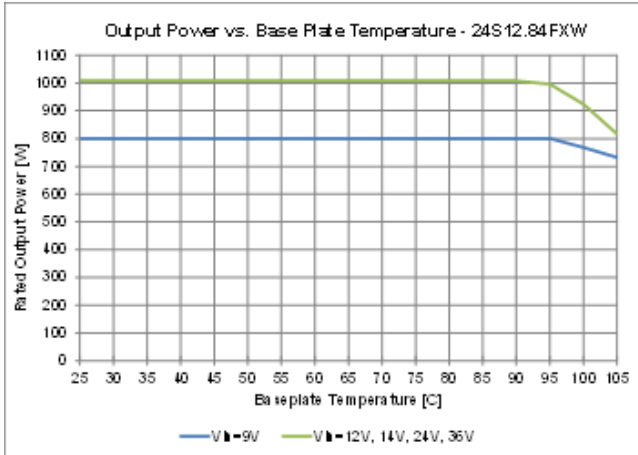
Figure 18: 24S12.84FXW (ROHS) Derating Curve
