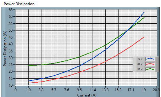
Figure 17: 24S53.19FXW (ROHS) Power Dissipation
