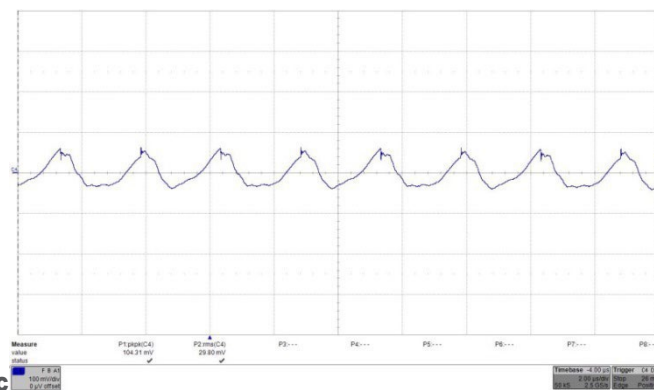
Figure 38: Output voltage ripple (100 mV/div.) at full rated load current into a resistive load at V_{in} = 24V . C_o = 2 \times 470 \mu F/70m\Omega . Time: 2 \mu s /div.
