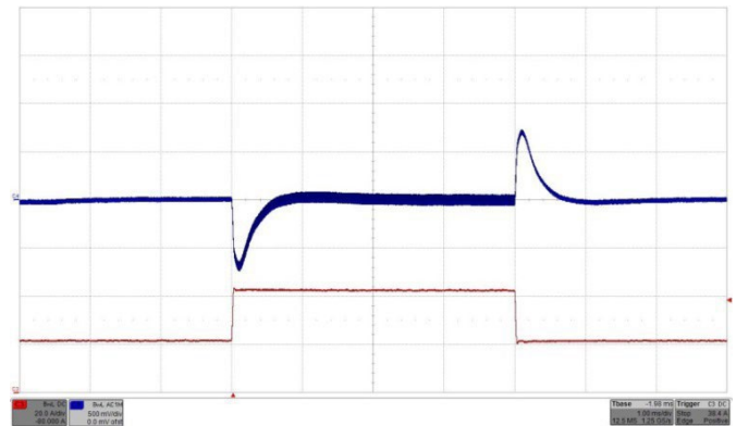
Figure 37: Output voltage response to load current step change 50% - 100% - 50% (21A–42A–21A) with di/dt = 1A/\mu s at V_{in} = 24V . Top trace (C4): Output voltage (500 mV/div.). Bottom trace (C3): Load current (20A/div.). C_o = 2 \times 470 \mu F/70m\Omega . Time: 1ms/div.
