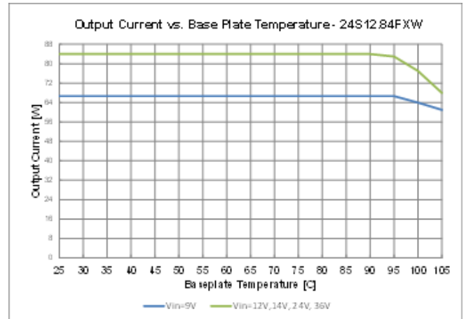
Figure 19: 24S12.84FXW (ROHS) Derating Curve
