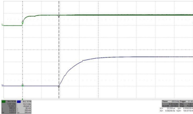
Figure 34: Turn-on by ON/OFF transient (with V_{in} applied) at full rated load current (resistive) at V_{in} = 24V . Top trace (C1): ON/OFF signal (5 V/div.). Bottom trace (C4): Output voltage (10 V/div.). Time: 5 ms/div.
