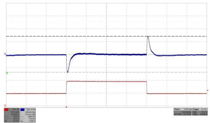
Figure 55: Output voltage response to load current step change 50% - 100% - 50% (9.5A–19A–9.5A) with di/dt = 1A/\mu s at V_{in} = 24V . Top trace (C4): Output voltage (500 mV/div.). Bottom trace (C3): Load current (10A/div.). Time: 1ms/div.
