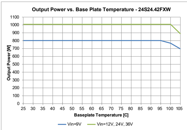
Figure 20: 24S24.42FXW (ROHS) Derating Curve
