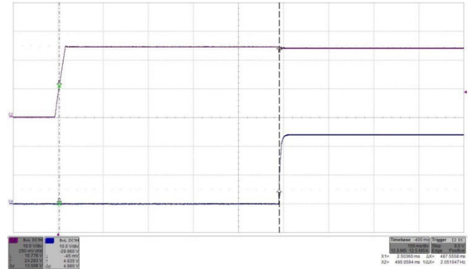
Figure 35: Turn-on by V_{in} transient (ON/OFF high) at full rated load current (resistive) at V_{in} = 24V . Top trace (C2): Input voltage V_{in} (10 V/div.). Bottom trace (C4): Output voltage (10 V/div.). Time: 100 ms/div.
