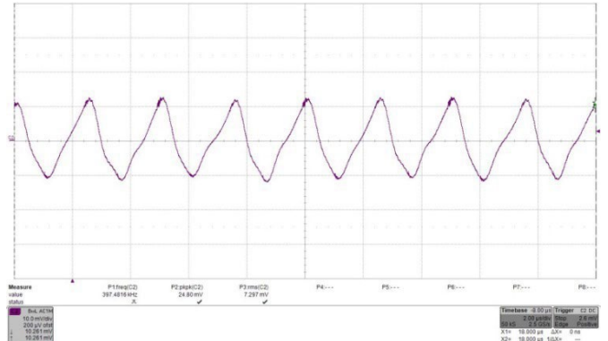
Figure 33: Input reflected ripple current, i_c (500mA/mV), measured at input terminals at full rated load current at V_{in} = 24V . Refer to Figure 3 for test setup. Time: 2 \mu s /div. RMS input ripple current is 7.3 \cdot 0.5A = 3.65A_{RMS} .
