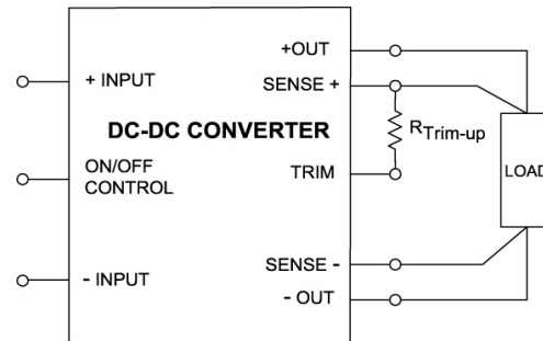
Figure 5: Circuit Configuration for Trim-Up Function
