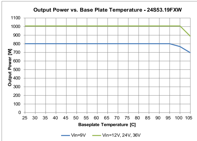
Figure 26: 24S53.19FXW (ROHS) Derating Curve
