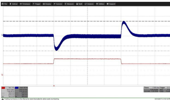
Figure 30: Output voltage response to load current step change 70% - 100%- 70% (58.5A–84A–58.8A) with di/dt = 0.5A/\mu s at V_{in} = 14V . Top trace (C4): Output voltage (200 mV/div.). Bottom trace (C3): Load current (50A/div.). Time: 1ms/div.
