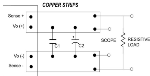
Figure 7: Test setup for measuring output voltage ripple, startup and step load transient waveforms
