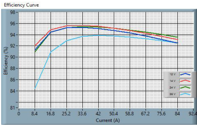
Figure 8: 24S12.84FXW (ROHS) Efficiency Curve
