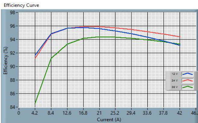
Figure 10: 24S24.42FXW (ROHS) Efficiency Curve
