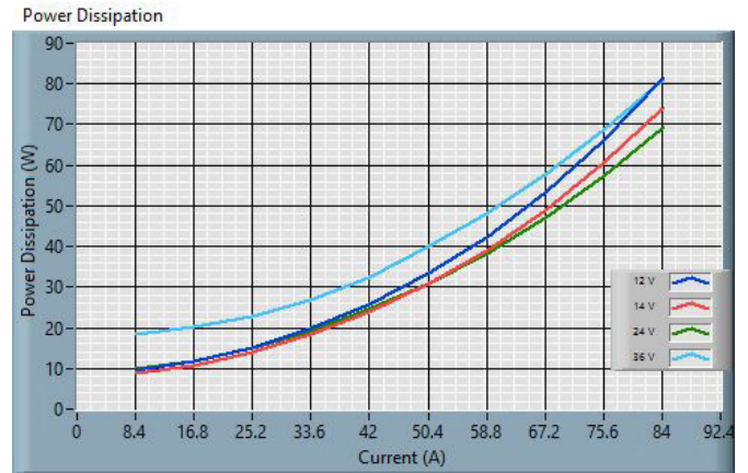
Figure 9: 24S12.84FXW (ROHS) Power Dissipation
