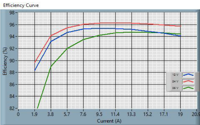
Figure 16: 24S53.19FXW (ROHS) Efficiency Curve
