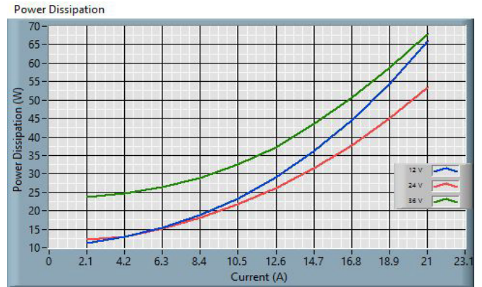
Figure 15: 24S48.21FXW (ROHS) Power Dissipation
