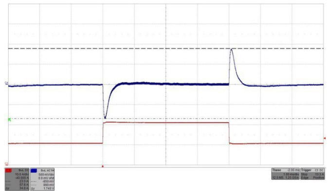
Figure 49: Output voltage response to load current step change 50% - 100%- 50% (10.5A–21A–10.5A) with di/dt = 1A/\mu s at V_{in} = 24V . Top trace (C4): Output voltage (500 mV/div.). Bottom trace (C3): Load current (10A/div.). Time: 1 ms/div.
