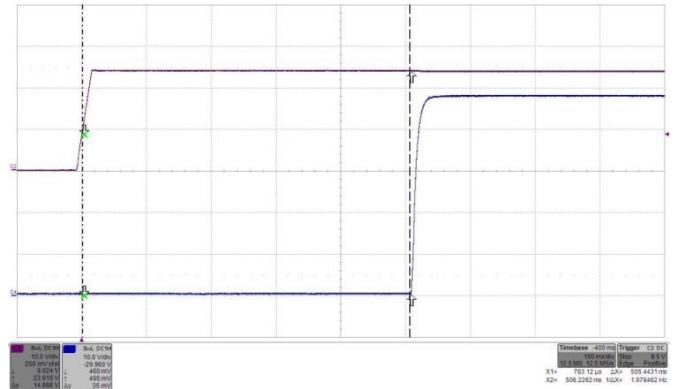
Figure 47: Turn-on by V_{in} (ON/OFF high) transient at full rated load current (resistive) at V_{in} = 24V . Top trace (C2): Input voltage V_{in} (10 V/div.). Bottom trace (C4): Output voltage (10 V/div.). Time: 100 ms/div.
