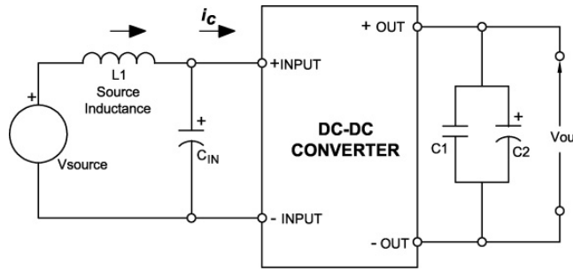
Figure 6: Test setup for measuring input reflected ripple currents
