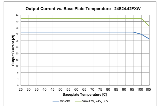
Figure 21: 24S24.42FXW (ROHS) Derating Curve
