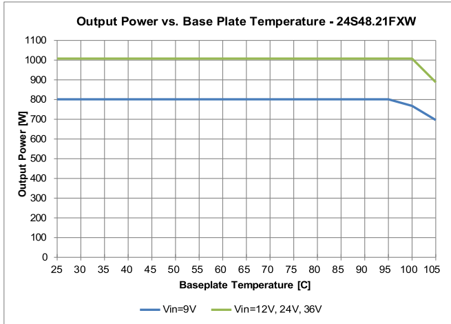
Figure 24: 24S48.21FXW (ROHS) Derating Curve
