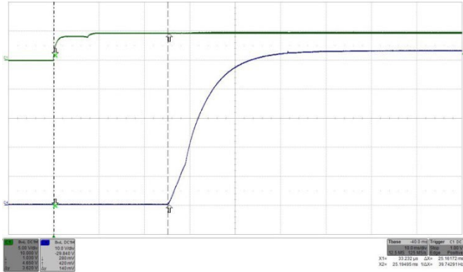
Figure 52: Turn-on by ON/OFF transient ( V_{in} applied) at full rated load current (resistive) at V_{in} = 24V . Top trace (C1): ON/OFF signal (5 V/div.). Bottom trace (C4): Output voltage (10 V/div.). Time: 10 ms/div.
