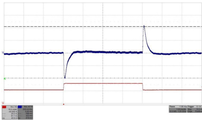
Fig. 4\87: Output voltage response to load current step change 50% - 75%- 50% (10.5A–15.75A–10.5A) with di/dt = 1A/\mu s at V_{in} = 24V . Top trace (C4): Output voltage (200 mV/div.). Bottom trace (C3): Load current (10A/div.). Time: 1 ms/div
