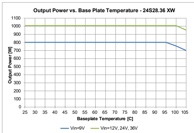
Figure 22: 24S28.36FXW (ROHS) Derating Curve
