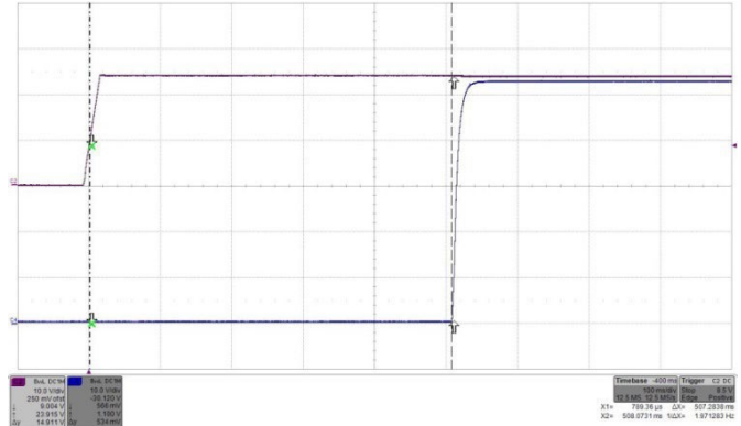
Figure 53: Turn-on by V_{in} (ON/OFF high) transient at full rated load current (resistive) at V_{in} = 24V . Top trace (C2): Input voltage V_{in} (10 V/div.). Bottom trace (C4): Output voltage (10 V/div.). Time: 100 ms/div.
