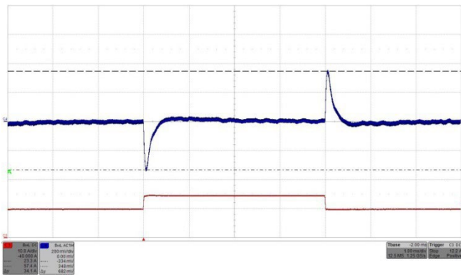
Figure 54: Output voltage response to load current step change 50% - 75% - 50% (9.5A–14.25A–9.5A) with di/dt = 1A/\mu s at V_{in} = 24V . Top trace (C4): Output voltage (200 mV/div.). Bottom trace (C3): Load current (10A/div.). Time: 1ms/div.
