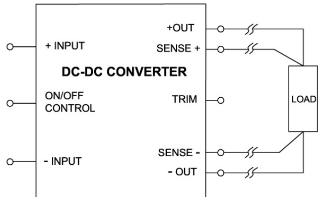
Figure 3: Circuit Configuration for Remote Sense Function
