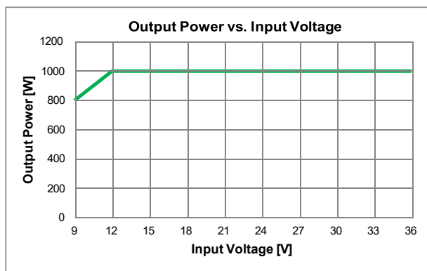
Figure 1: Output Power as Function of Input Voltage
