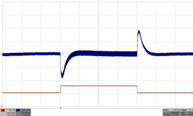
Figure 36: Output voltage response to load current step change 50% - 75% - 50% (21A–31.5A–21A) with di/dt = 1A/\mu s at V_{in} = 24V . Top trace (C4): Output voltage (200 mV/div.). Bottom trace (C3): Load current (20A/div.). C_o = 470\mu F/70m\Omega . Time: 1ms/div.
