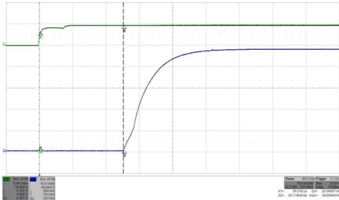
Figure 46: Turn-on by ON/OFF transient ( V_{in} applied) at full rated load current (resistive) at V_{in} = 24V . Top trace (C1): ON/OFF signal (5 V/div.). Bottom trace (C4): Output voltage (10 V/div.). Time: 10 ms/div..
