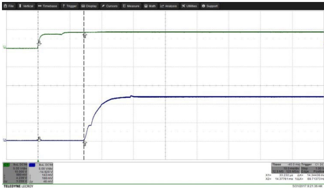
Figure 28: Turn-on by ON/OFF transient (with V_{in} applied) at full rated load current (resistive) at V_{in} = 14V . Top trace (C1): ON/OFF signal (5 V/div.). Bottom trace (C4): Output voltage (5 V/div.). Time: 10 ms/div.
