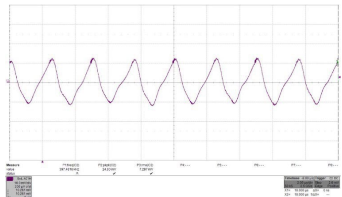
Figure 39: Input reflected ripple current, i_c (500mA/mV), measured at input terminals at full rated load current at V_{in} = 24V . Refer to Figure 3 for test setup. Time: 2 \mu s /div. RMS input ripple current is 7.3 \times 0.5A = 3.65A_{RMS} .
