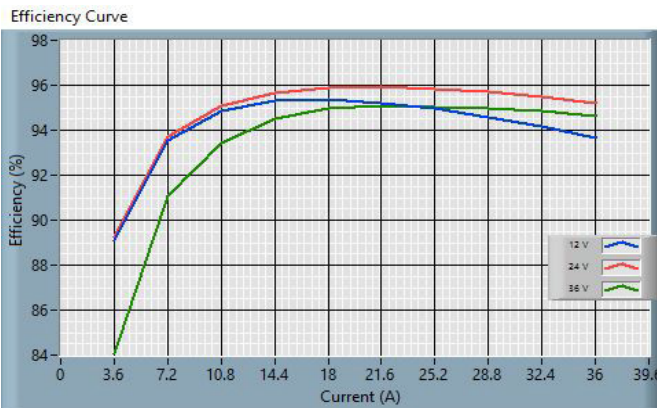
Figure 12: 24S28.36FXW (ROHS) Efficiency Curve
