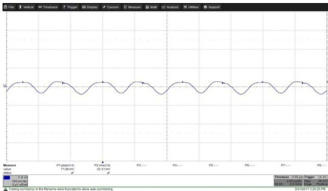
Figure 32: Output voltage ripple (100 mV/div.) at full rated load current into a resistive load at V_{in} = 14V . Time: 2 \mu s /div
