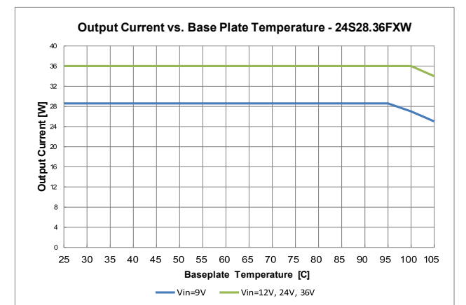
Figure 23: 24S28.36FXW (ROHS) Derating Curve
