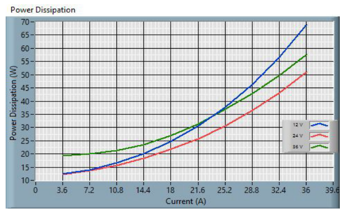
Figure 13: 24S28.36FXW (ROHS) Power Dissipation
