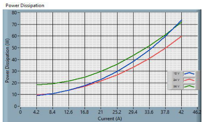
Figure 11: 24S24.42FXW (ROHS) Power Dissipation
