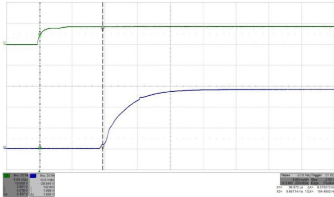
Figure 40: Turn-on by ON/OFF transient ( V_{in} applied) at full rated load current (resistive) at V_{in} = 24V . Top trace (C1): ON/OFF signal (5 V/div.). Bottom trace (C4): Output voltage (10 V/div.). Time: 5 ms/div.
