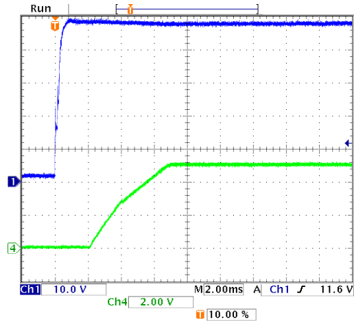
Power On Startup Delay (Vin=0 to 48V, Vout=nom, Iout=10A, Cload=0 uF, Ta=+25°C., Scope BW=20MHz) Trace 1=Vin, Trace 4=Vout
