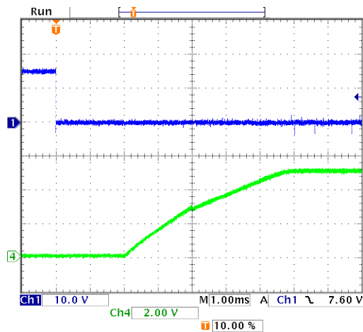
On/Off Enable Delay (Vin=48V, Vout=nom, Iout=10A, Cload=0 uF, Ta=+25°C., Scope BW=20MHz) Trace 1=Enable, Trace 4=Vout
