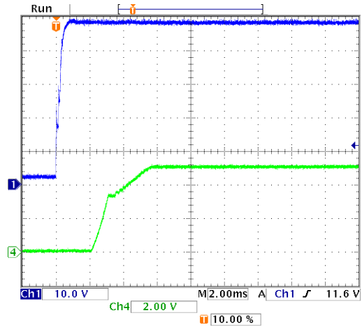
Power On Startup Delay (Vin=0 to 48V, Vout=nom, Iout=0A, Cload=0 uF, Ta=+25°C., Scope BW=20MHz) Trace 1=Vin, Trace 4=Vout
